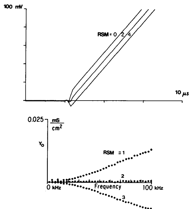
FIGURE 1 Measurement of a known 2\text{ }\Omega\text{cm}^2 R_s by: (A) minimizing the voltage jump across a 2\text{ }\Omega\text{cm}^2 RC model membrane in response to a current step at various settings of the RSM potentiometer (see Fig. 3) and by (B) finding the value of the R_s measurement (RSM potentiometer) for which the measured in-phase or conductive admittance, Y_o , is frequency independent. Each tick mark on the abscissa equals 10\text{ }\mu\text{s} /mark.
