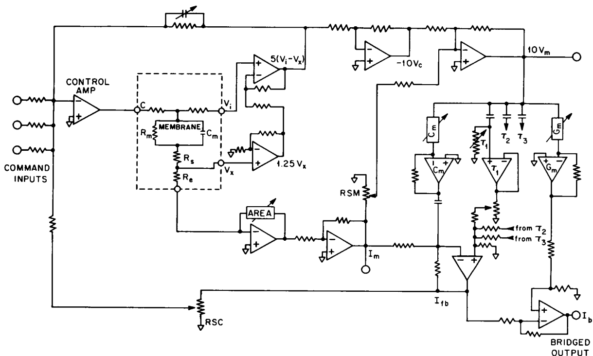
FIGURE 3 Schematic diagram of voltage-clamp circuit showing methods of measuring and full compensation for the R_s with the membrane. The active bridge circuit (right) develops signals to balance (subtract) the currents through normal 1 \mu\text{F}/\text{cm}^2 capacitance ( C_m ), the leakage resistance ( G_m ), and the nonideal Cole-Cole capacitance with three time constants. The amplifier circuits for \tau_2 and \tau_3 are identical to that for \tau_1 and are not shown.
